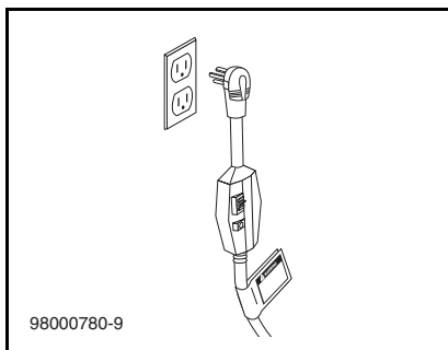
STEP 2: Connect the power cord into the proper electrical outlet, then push in the GFCI reset button. (Refer to serial plate for information).
